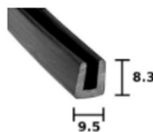
Fits 5.5 - 6mm Material
